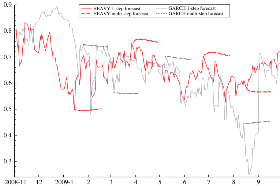
Figure 3. One-step and multi-step forecasts for the SPY-BAC conditional correlation. This figure is available in color online at wileyonlinelibrary.com/journal/jae
