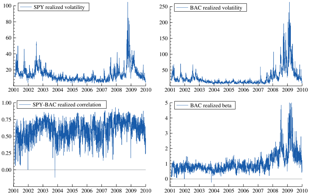
Figure 1. SPY and BAC annualized realized volatility, realized correlation and BAC realized beta. This figure is available in color online at wileyonlinelibrary.com/journal/jae
