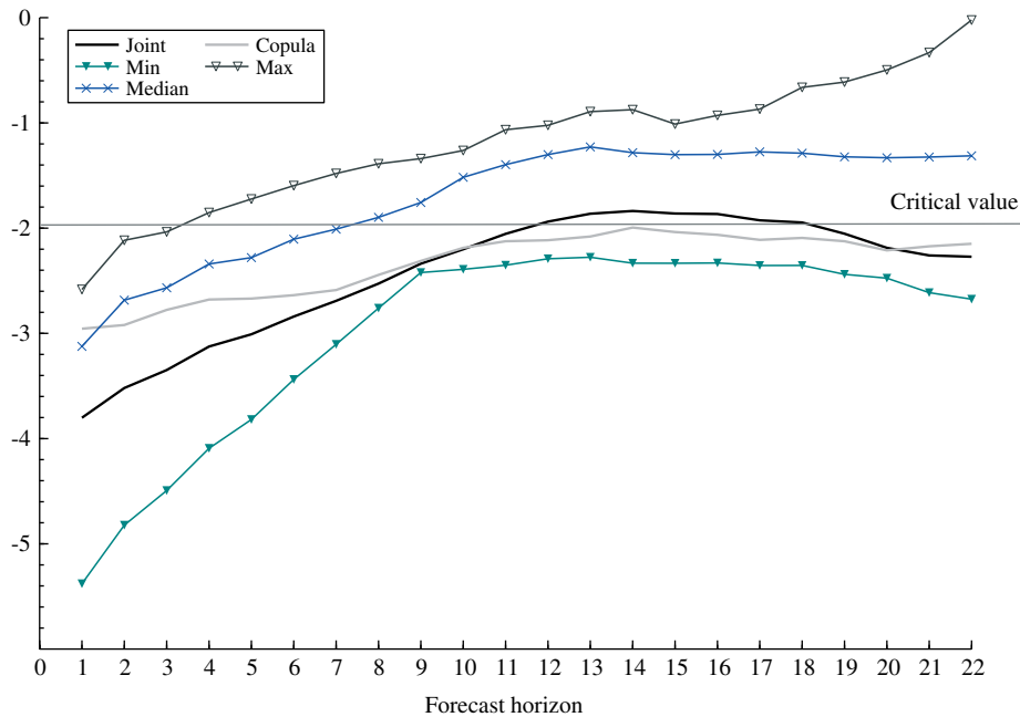
Figure 4. Predictive ability tests' t -statistics for the covariance targeting scalar HEAVY and GARCH models. This figure is available in color online at wileyonlinelibrary.com/journal/jae
