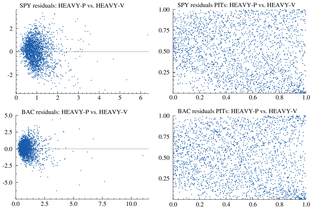
Figure 2. Left: scatter-plots of SPY and BAC residuals in the HEAVY-P and HEAVY-V equations. Right: scatter-plots of the residuals mapped into probability integral transforms (PITs). This figure is available in color online at wileyonlinelibrary.com/journal/jae
