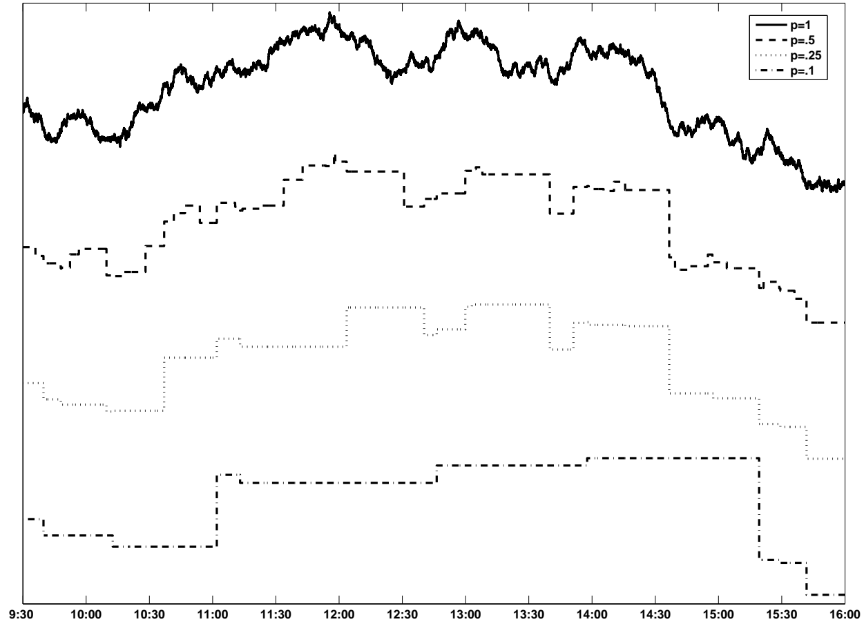
Figure 5: These four series show the evolution of prices as the probability of no trade using a 5-minute windows decreases from 1 through .5, and .25 to .1. All series were constructed using the same random data. The variance of the daily return was set to be 1.
