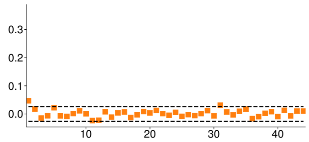
Std. Squared Residuals PACF
