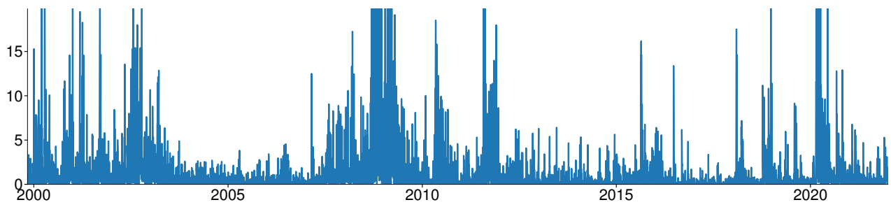
Squared WTI Returns
