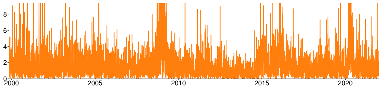
Absolute WTI Returns
