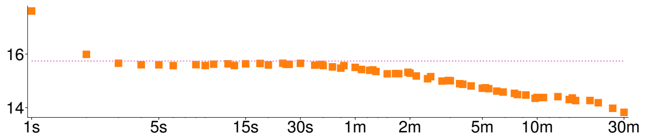
Volatility Signature Plot for SPDR RV^{AC1}
