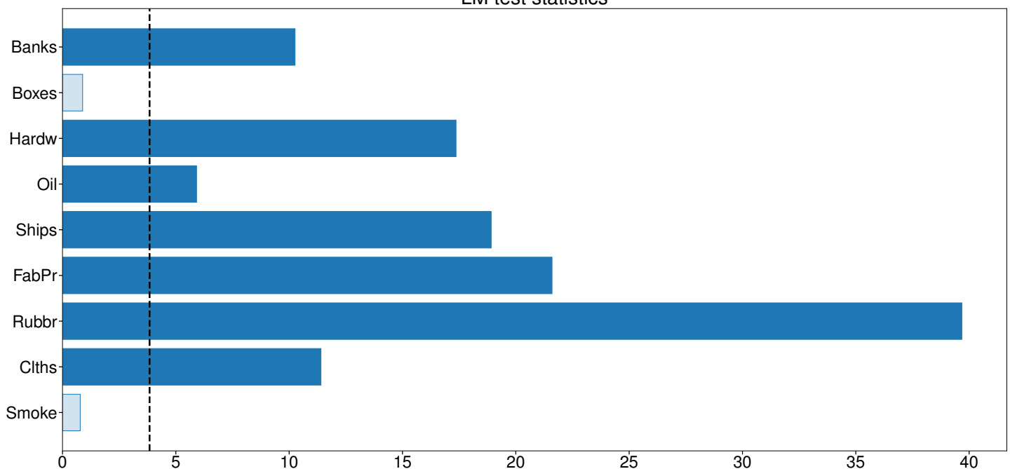
LM test statistics
